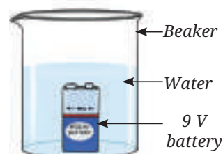
(b) 9 V battery placed inside the beaker containing water
