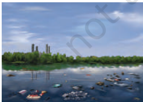
Fig. 13.16: Water pollution
